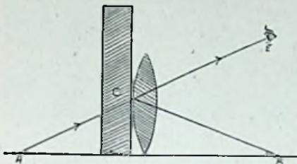
VIEWING COLOURS OF GREATER BRILLIANCE BY ARAGO'S EXPERIMENT
