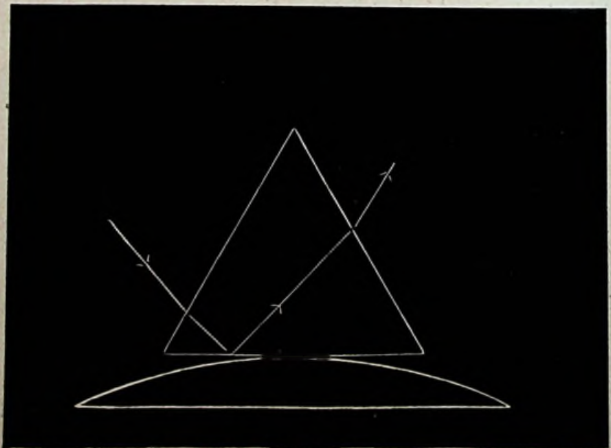
Newton's method for viewing a greater number of coloured rings. Fig. 4.
