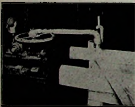
The recording turntable of the phonovision apparatus in the Baird Laboratories.
