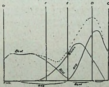
DIAGRAMMATIC RESULTS OF MAXWELL'S COLOUR CALCULATIONS
