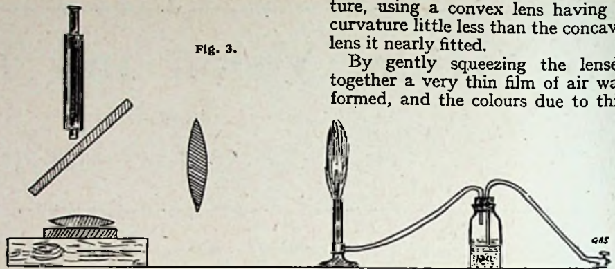
NEWTON'S METHOD OF OBSERVING RINGS.
