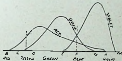
THREE SETS OF PRIMARY NERVES ARE STIMULATED BY LUMINOUS RAYS OF DIFFERENT WAVELENGTH
